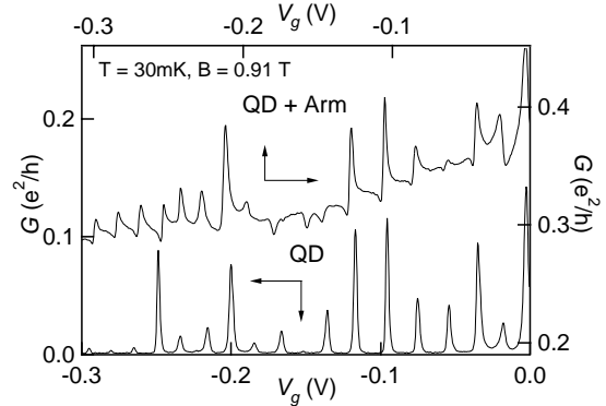
Fig. 2. Typical Coulomb oscillation at V_C = -0.12 \text{ V} with the arm pinched off, and asymmetric Coulomb oscillation at V_C = -0.086 \text{ V} with the arm transmissible. The latter shows a clear Fano effect. Both of them were obtained at T = 30 \text{ mK} and B = 0.91 \text{ T} .
