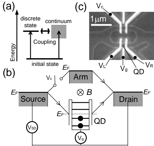
Fig. 1. (a) The principle of the Fano effect. (b) Schematic representation of the experimental setup. (c) Scanning electron micrograph of the correspondent device fabricated by wet-etching the 2DEG at an AlGaAs/GaAs heterostructure. The three gates ( V_R , V_L , and V_g ) at the lower arm are used for controlling the QD and the gate at the upper arm is for V_C .
