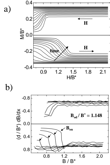
Fig. 2. Numerical calculation of (a) global magnetic moment M(H) and (b) local dB/dx(B) for different times. Arrows in (b) point to the onset of the SMP at B_{on} .
