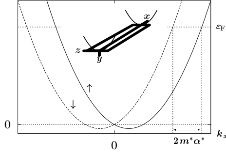
Fig. 1. Energy dispersion in the lowest spin split subband of a quantum wire. On the wire axis the spins s = \uparrow, \downarrow are polarized in the plane of the heterostructure parallel to the z -direction.
