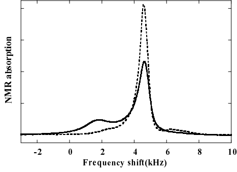
Fig. 1. NMR absorption line shapes for the 0.2mm sample at T/T_c = 0.75 as function of frequency shift from Lari frequency. The dotted line was taken at rest and the solid was taken at rotation speed of 6.28 rad/sec.
