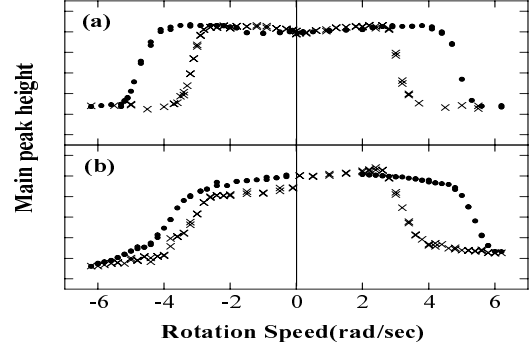
Fig. 2. NMR absorption at R_t^2 = 1 during acceleration (solid circle) and deceleration (cross). (a): the sample was cooled to superfluid at rest and (b): it was cooled under the rotation speed of +2 rad/sec
