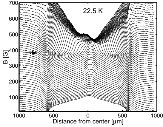
Fig. 1. Induction profiles in BSCCO at T=22.5 K, measured during decrease of the external field from 850 to 0 G at a rate of 6 G/sec. The arrow marks the induction at the break appearing at 380 G.
