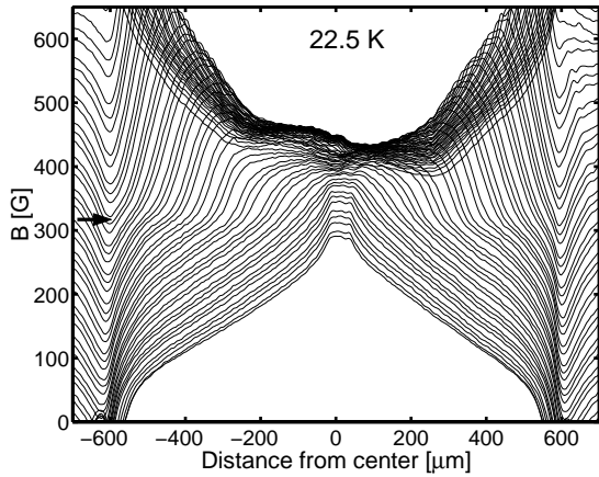
Fig. 2. Induction profiles in BSCCO at T=22.5 K, measured during decrease of the external field from 850 to 0 G at a rate of 47.6 G/sec. The arrow marks the induction at the break appearing at 320 G.
