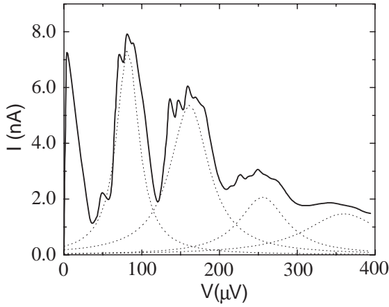
Fig. 1. IV-curve in the subgap region for the maximum value of E_J/E_C = 50 . The dotted curves show the fitted resonances to the series of peaks. The measurements were carried out at 100 mK.
