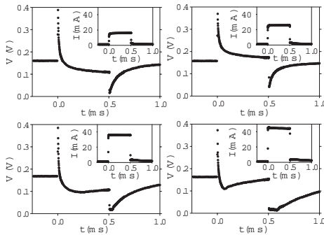
Fig. 3. Sample voltage and (inset) current for pulses with a low applied level of 0.5 V and 500 \mu\text{s} high applied levels of (a) 2 V, (b) 3 V, (c) 4 V and (d) 5 V, at a base temperature of 23 K. Note the small size of the current at low bias compared to its high-bias values.
