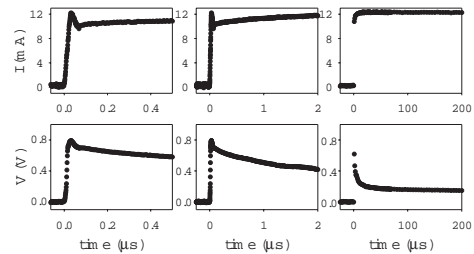
Fig. 1. Variation of sample current and voltage at 9 K for an applied simple square pulse of 4 V.
