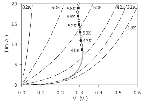
Fig. 4. IV characteristics just before the end of the 5 \mu\text{s} high-bias pulse (circle symbols), at a base temperature of 18 K. The solid line is a guide for the eye. The labels beside alternate points (filled circles) indicate the temperature just after the end of the high-bias pulse, inferred from the resistance of the stack during the low level. Dashed lines show fits to 50 ns IV characteristics at a number of base temperatures.
