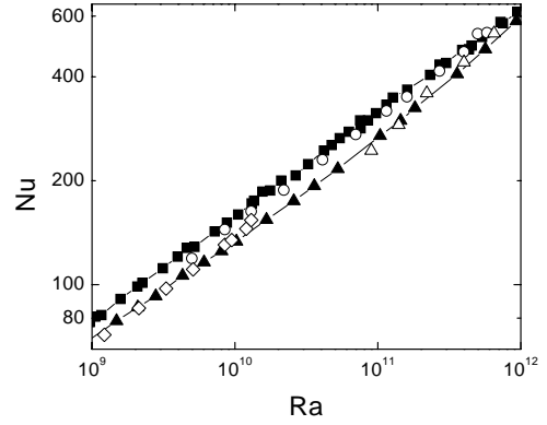
Fig. 1. Nu vs Ra . Filled squares, ref.[1]; filled triangles, ref.[7]; open symbols, ref.[8]. There appear to be two main branches of Nu consistent with the existence of two distinct modes of the LSC.
