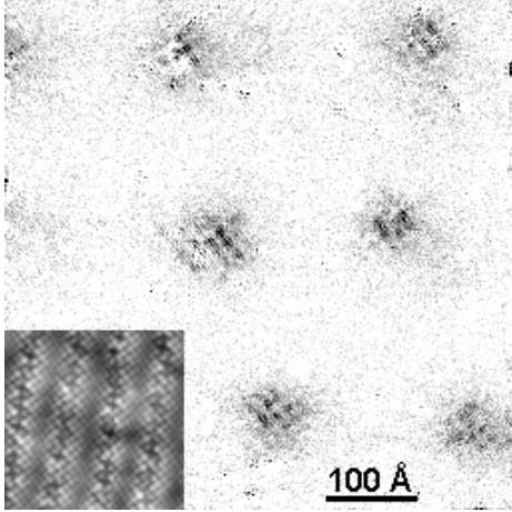
Fig. 1. Map of S_1^{12}(x, y, 5) : seven vortices are evident as the darker regions of dimension \sim 100 Å with an internal ‘checkerboard’ pattern. The inset shows a topographic image of the BiO plane at 2\times magnification. The atomically resolved square lattice and the supermodulation at 45^\circ are evident.
