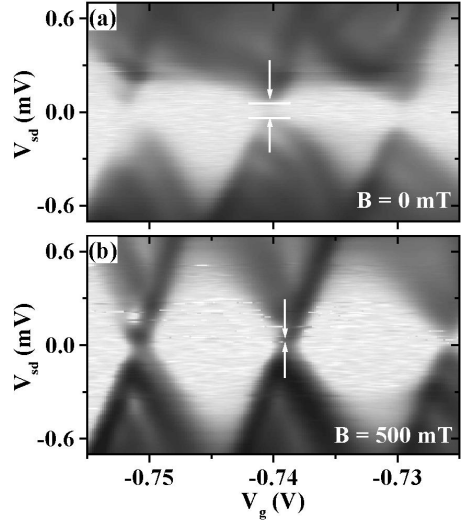
Fig. 2. (a) Coulomb blockade in a freely suspended quantum dot. The observed energy gap is marked by arrows. (b) At a magnetic field of B = 500 \text{ mT} linear transport is re-established.
