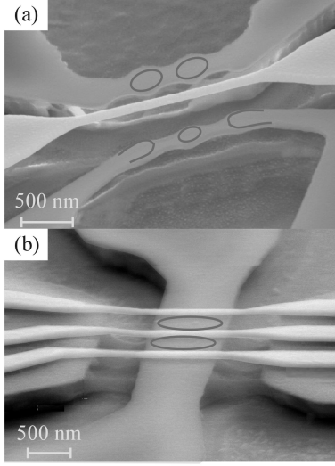
Fig. 1. Freely suspended quantum dot structures defined by (a) symmetric indentations (b) crossing gate electrodes.
